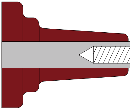
Interface C (bolted type 400 series)
