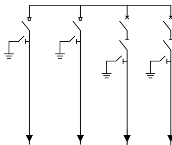
CCVV Depth: 900 mm Width: 1750 mm Height: 1930 mm
