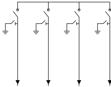
CCCC Depth: 900 mm Width: 1750 mm Height: 1930 mm
