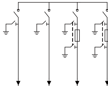
CCFF Depth: 900 mm Width: 1750 mm Height: 1930 mm
