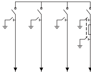
CCCF Depth: 900 mm Width: 1750 mm Height: 1930 mm
