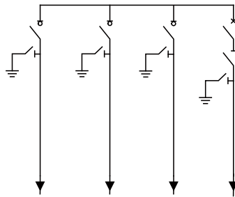
CCCV Depth: 900 mm Width: 1750 mm Height: 1930 mm
